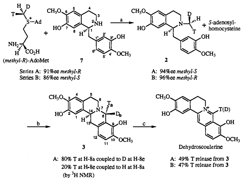
Figure 1. Biosynthetic pathway to berberine in Berberis cell cultures.
