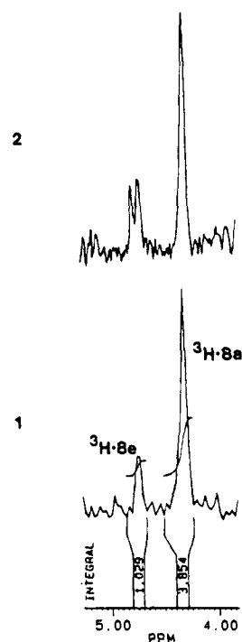
Figure 3. Tritium NMR spectra of scoulerine ( 3 ) generated from ( methyl-S )-[ methyl-2 H 1 , 3 H]- 2 with BBE. Sample contained 153 μCi 3 H, solvent CD 3 OD, repetition time 1.0 s; spectrum 1, composite pulse broadband 1 H-decoupled, 76472 acquisitions; spectrum 2, 1 H-decoupler gated off during acquisition, WALTZ-16 2 H broadband decoupled, 47 347 acquisitions.
