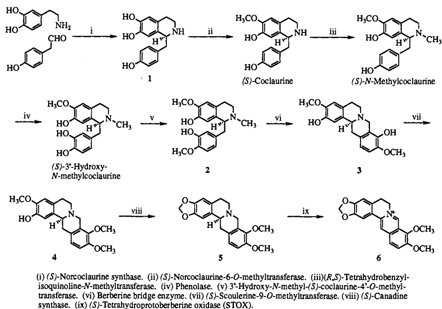
Figure 1. Biosynthetic pathway to berberine in Berberis cell cultures.
