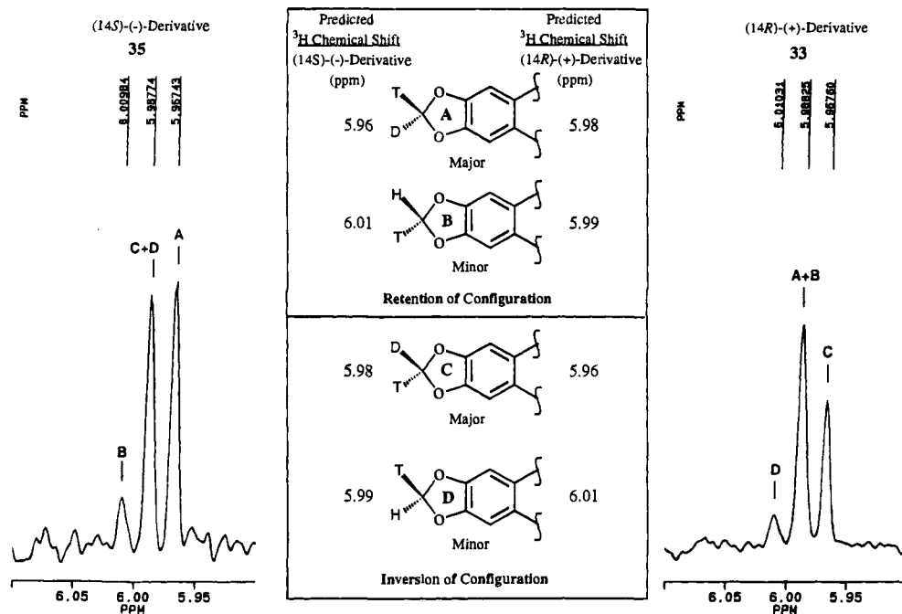
Figure 4. Proton-decoupled tritium NMR spectra of (+)- and (-)-canadine derivatives 33 and 35 . The samples contained 270 and 300 \mu\text{Ci} of tritium, respectively; the solvent was \text{CDCl}_3 . Predicted ^3\text{H} chemical shifts are based on the ^1\text{H} chemical shifts and the observed deuterium isotope shift is based on the ^3\text{H} signal in 31 .
