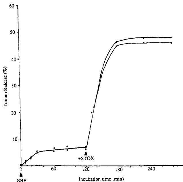
Figure 2. Tritium release in the formation of the berberine bridge by BBE and its dehydrogenation by STOX with ( methyl-R )-[ methyl-2 H 1 , 3 H]- 2 (●) and ( methyl-S )-[ methyl-2 H 1 , 3 H]- 2 (○) as substrate. The incubations contained 4.2 nmol of 2 (0.67 and 0.42 μCi, respectively) and 0.25 pkat of BBE. Samples were analyzed for tritium released into the solvent at the times indicated. At 120 min, 5 pkat of STOX were added, and the analyses were continued.
